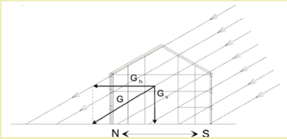
Figure 2: Relative horizontal and vertical components of solar radiation.
