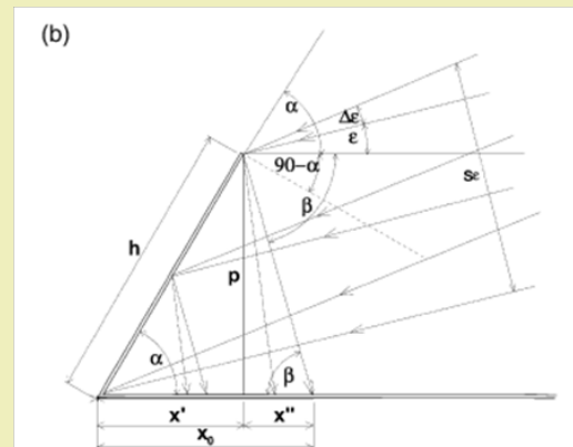
Figure 4: Schematic representations of (a) diffuse light falling onto a point at distance x/h from the reflecting wall, and of (b) diffuse light reflected by the wall.
